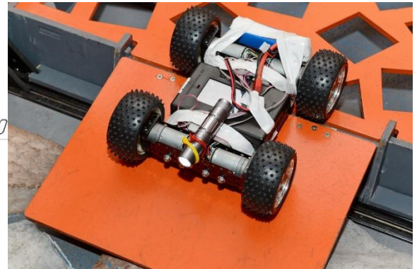
Figure 5. 20° Inclined Surface
