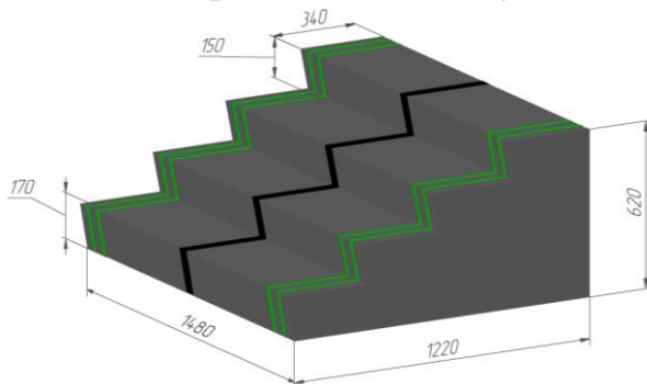
Figure 30. Staircase
