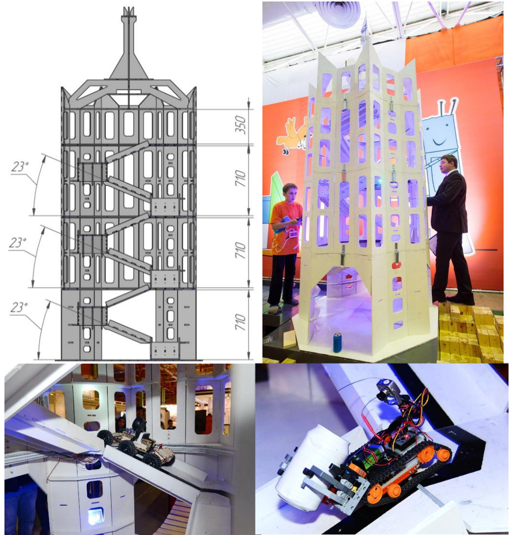
Figure 33. Tower
