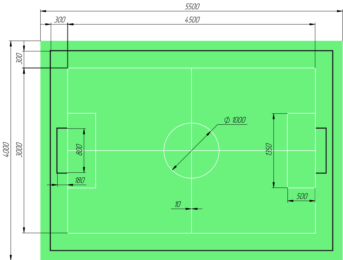
Figure 1. Field dimensions and markings for division C
